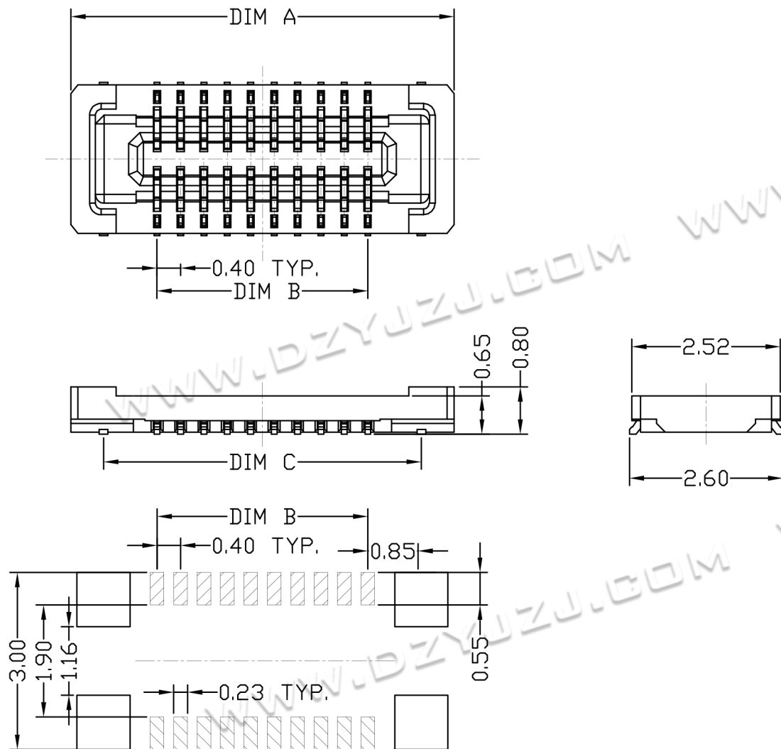
RECOMMENDED PCB LAYOUT CONNECTOR SIDE
